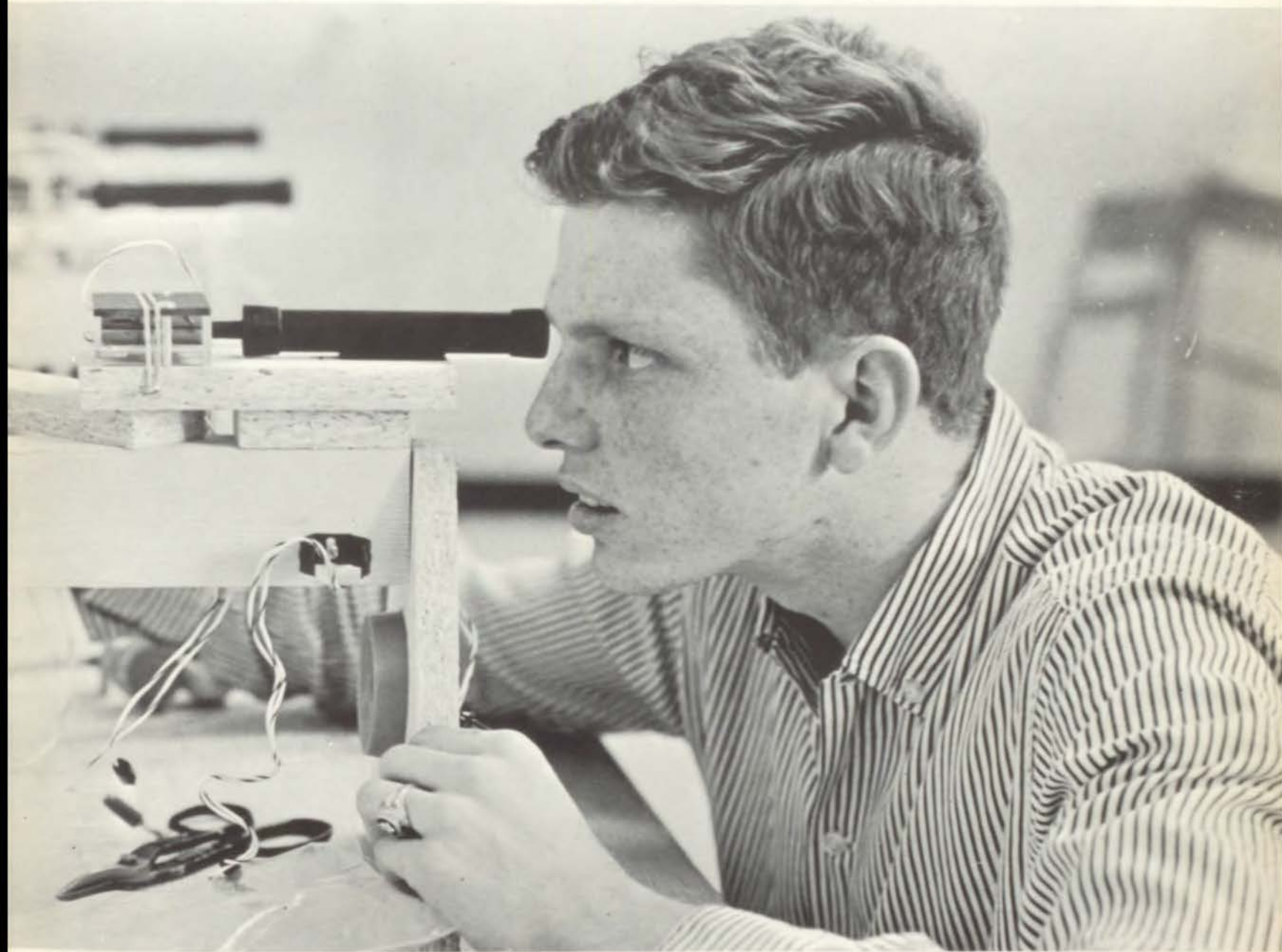
Allen Fickling observes a floating particle in motion during a physics experiment.
